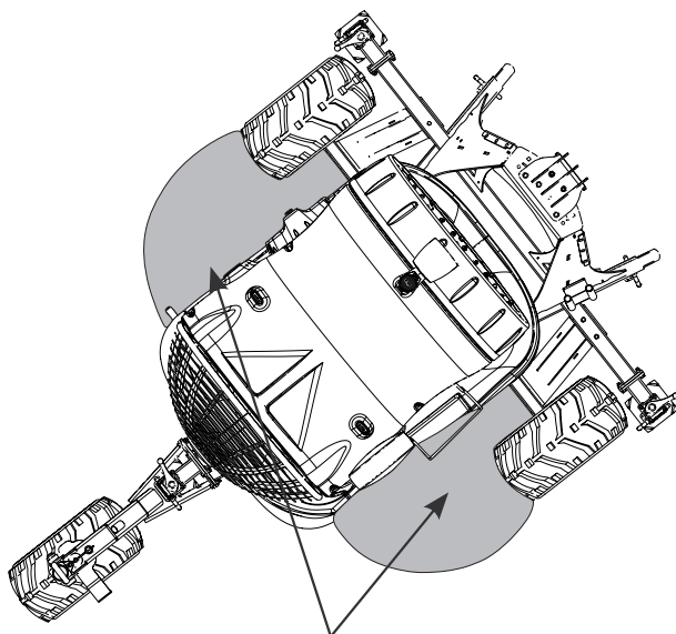
Permissible area occupied by the operator when working with a machine
