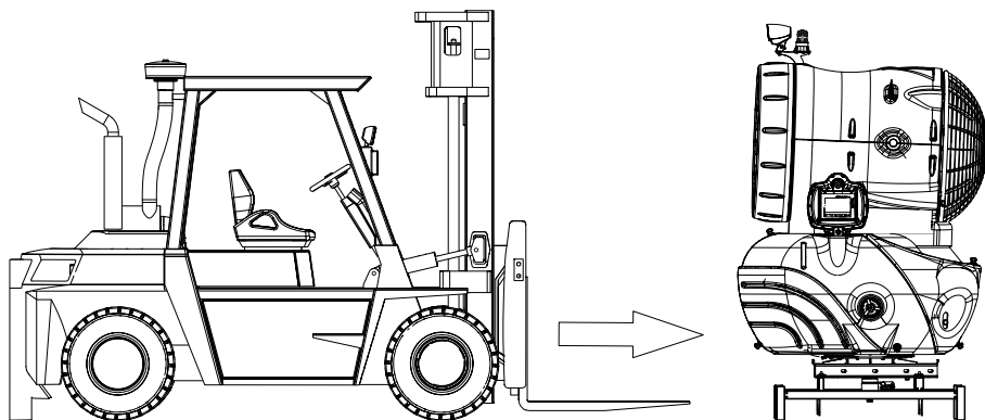
The method of transporting the snow gun with a forklift
