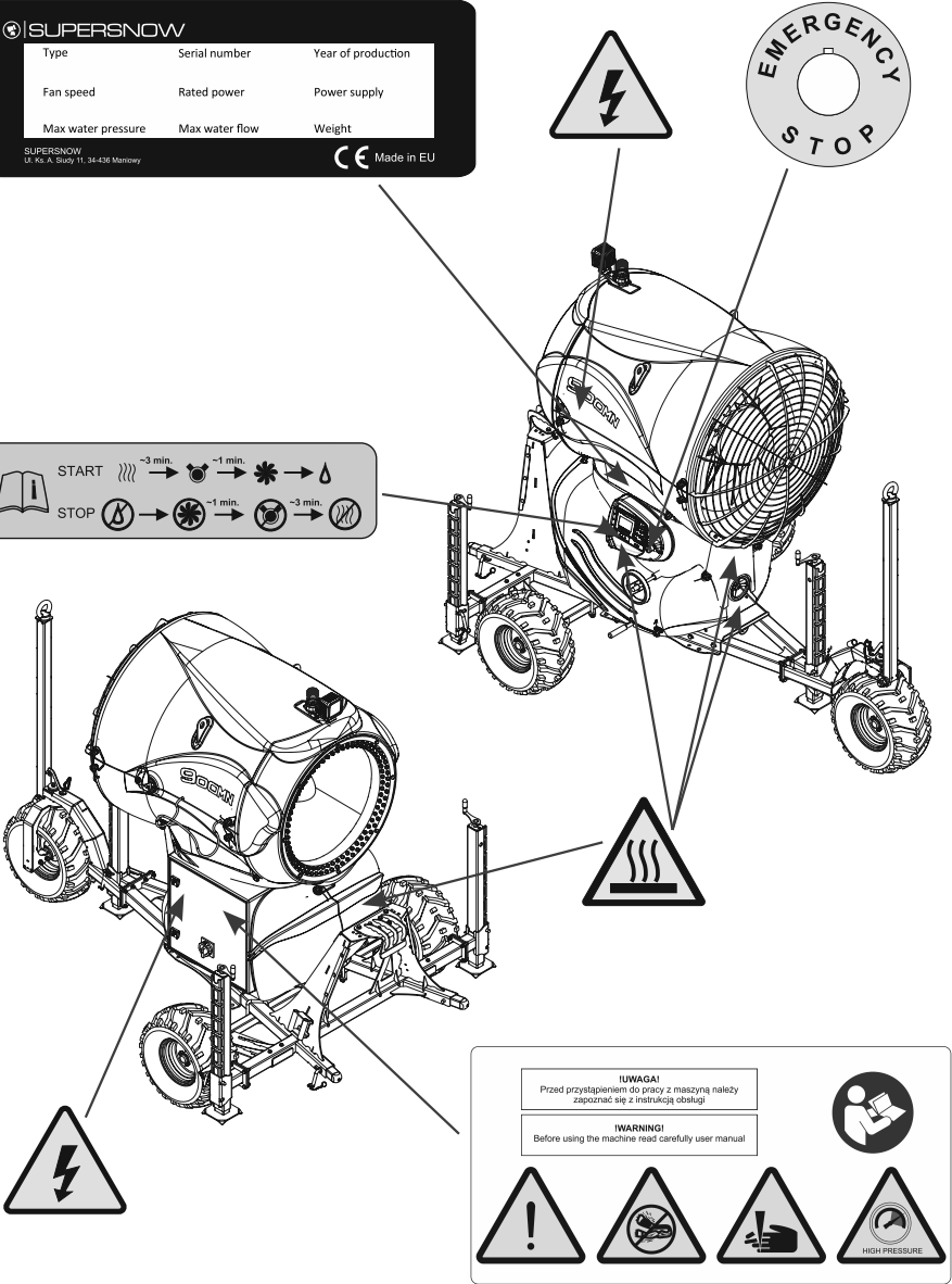
Location of warning and information labels in the 900MN snow gun
