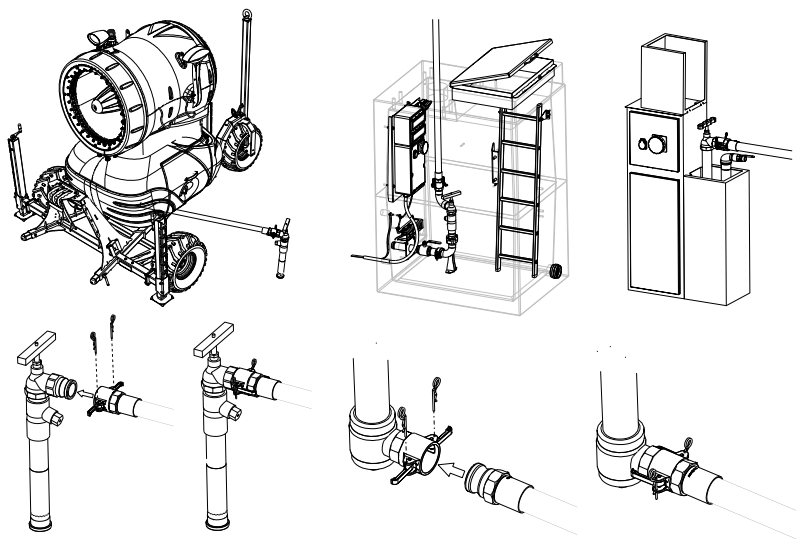
The diagram for a water feeding hose installation
