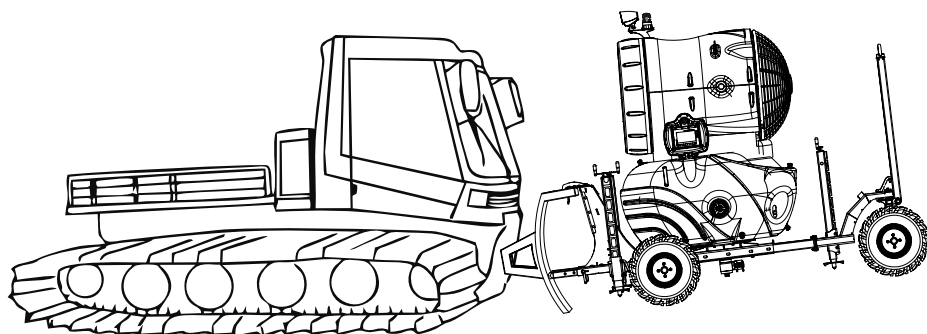
Method of transporting a snow gun on the snow groomer's blade
