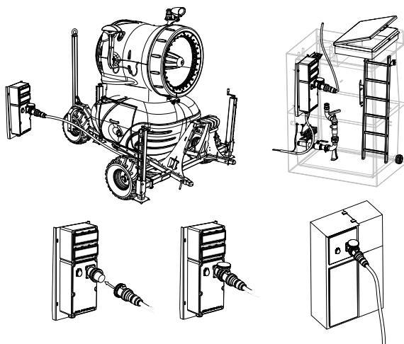
Diagram of connecting the electrical supply (CEE 63A connector) of the snow gun to the electric box on the slope and installation in the well
