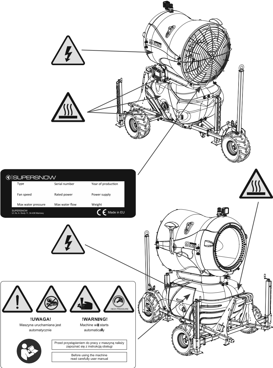
Location of warning and information labels in the 900A snow gun
