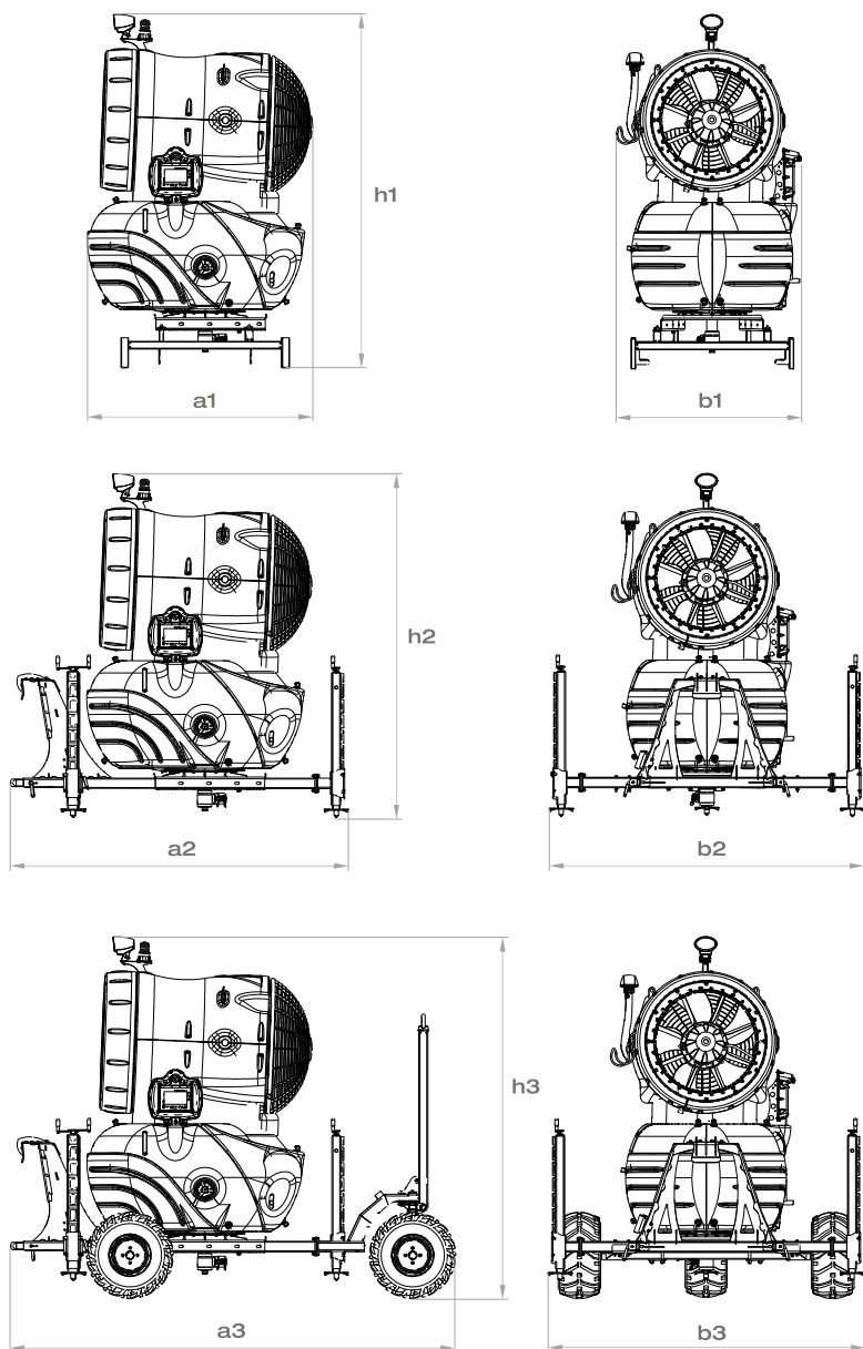
Dimensions of snow guns on various chassis
