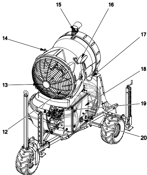
Construction of the snow gun
