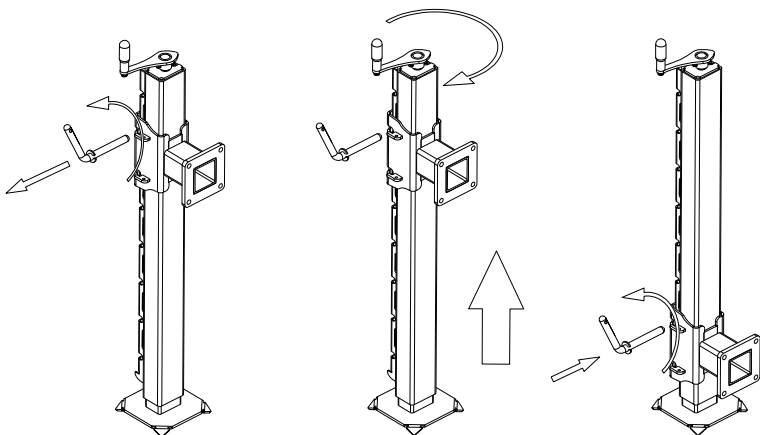
"feet" lift scheme
