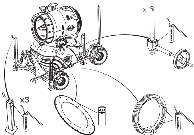
Points for periodic lubrication of the snow gun
