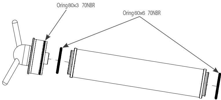
O-rings that require checking when cleaning the water filter (*700H, 700S)
