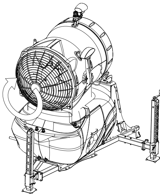
The correct direction of the fan rotation
