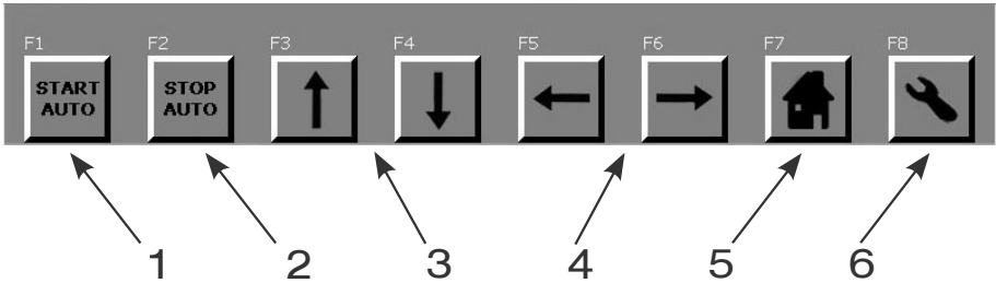
7.3.2. 700ASE, 700H, 700S, 900A control panel icons
