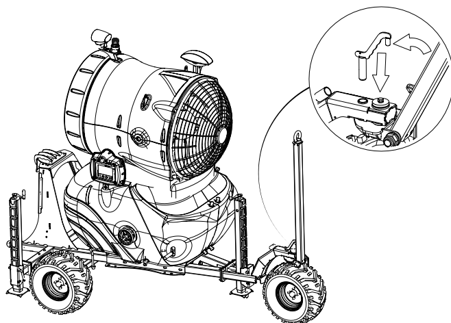
Method of securing the drawbar after towing
