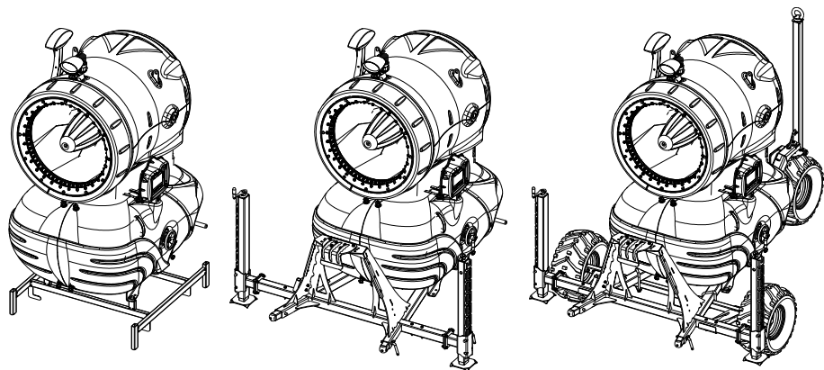
Snow gun (on the left) on the technological basis, on the feet chassis, on the wheel chassis
