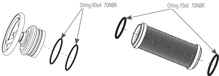
O-rings that require checking when cleaning the water filter (*600M, 900MN, 700A SE, 900A)
