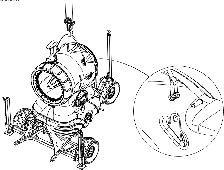
Location of the snow gun transport handles
